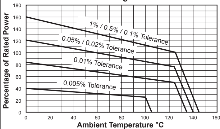
FIGURE 2 – DERATING
