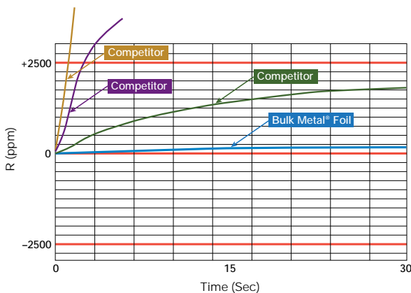
Figure 3. Thermal stabilization demonstration (1 W applied to 50 m SMD 2512)
