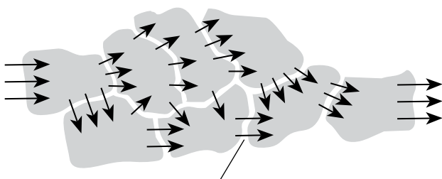
Figure 22. The Current Path in a Resistive Alloy
