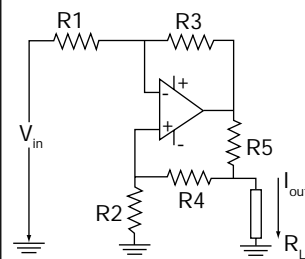
Diagram 8: High Common Mode Voltage Rejection Unity Gain Differential Amplifier
