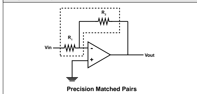
Figure 2. Typical Application
