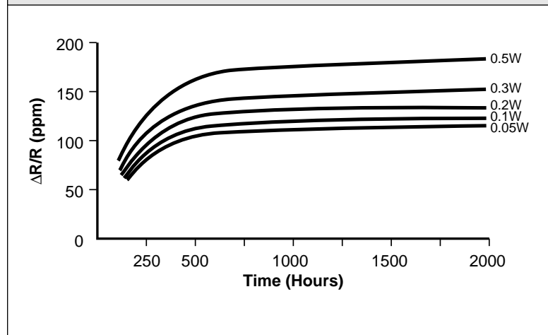
Figure 1. (\Delta R/R) = F(\text{Time}) , Loads 0.05 to 0.5W, +125°C Ambient
