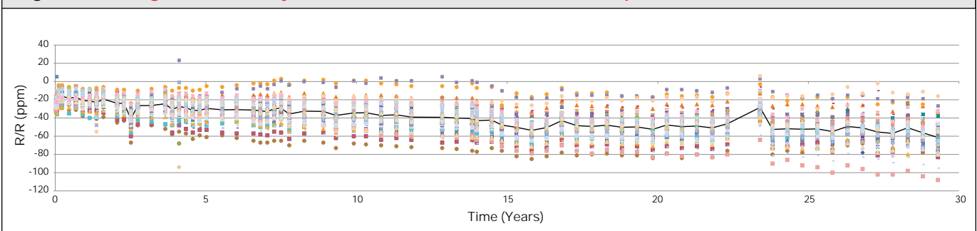
Figure 10. Long-Term Stability Over 29 Years, 0.1W at 70°C, 50 Samples (S102C, 10 K \Omega )
