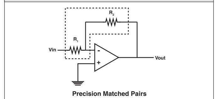
Figure 2. Typical Application
