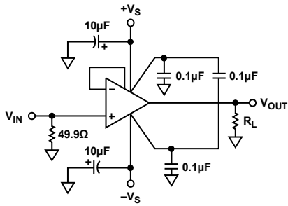
Figure 42. Noninverting Load Configuration
