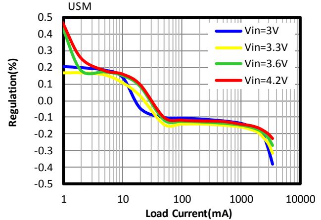
Load Regulation
