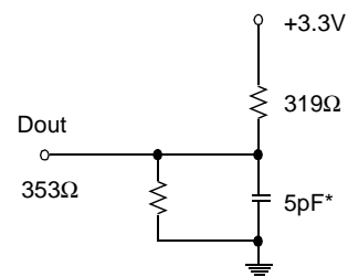
Output Load(B) (for tLZC, tLZOE, tHZOE & tHZC)
