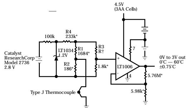
Total Power Consumption \leq 500\mu W * = TRW MAR-60.1% R1 = Yellow Springs Inst. Co Model 44007 5k @25°C
