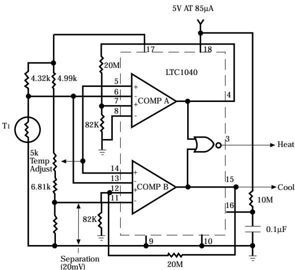
T1 Thermistor #44007 Yellow Springs Instrument Co., Inc. Hysteresis = 5V \times 82k = 20mV 20M
