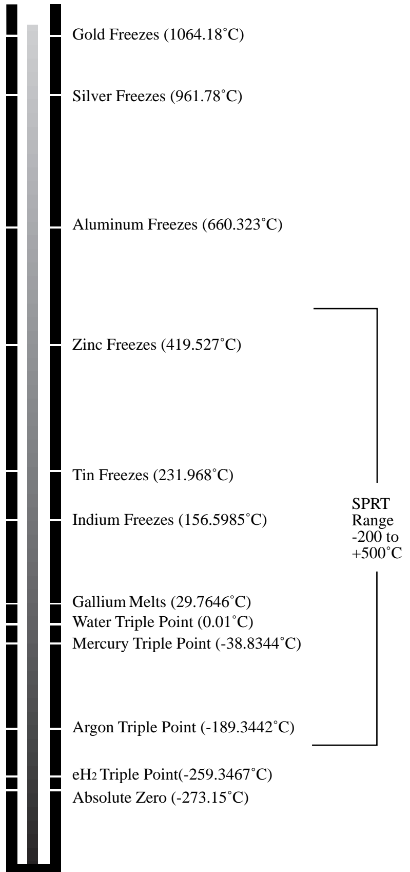
ITS-90 Scale
