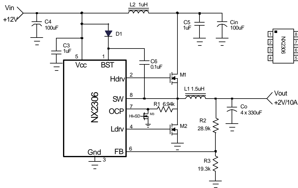
Figure 1 - Typical application of 2306
