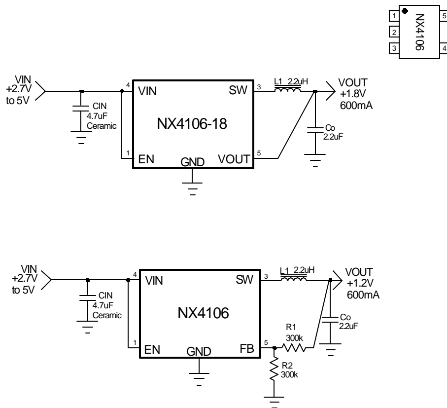
Figure 1 - Typical application of 4106-18 and 4106
