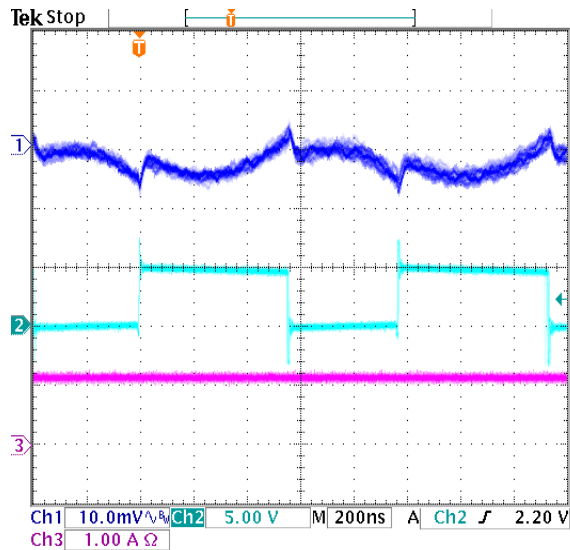
Fig.6 Output ripple @1A
