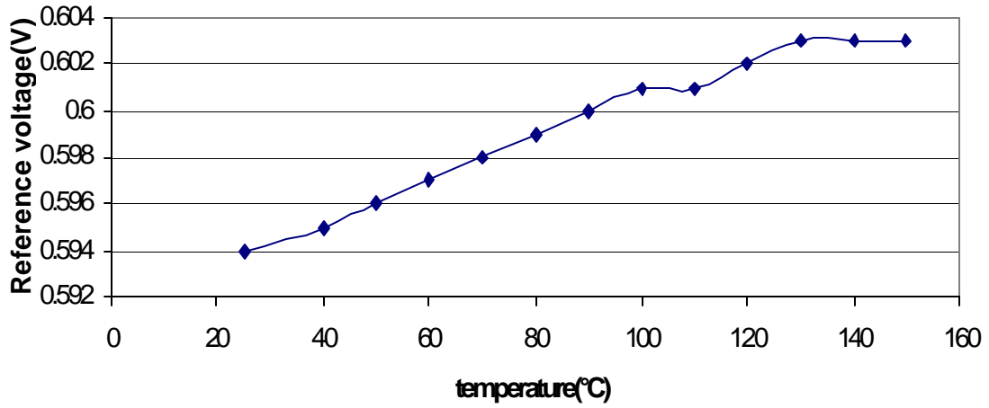
Fig.3 Reference volateg vs temperature
