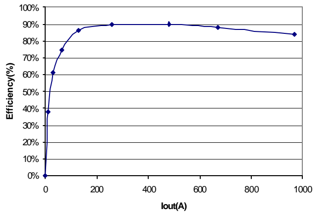
Fig.9 Efficiency
