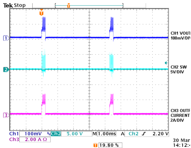
Fig.8 Short circuit protection
