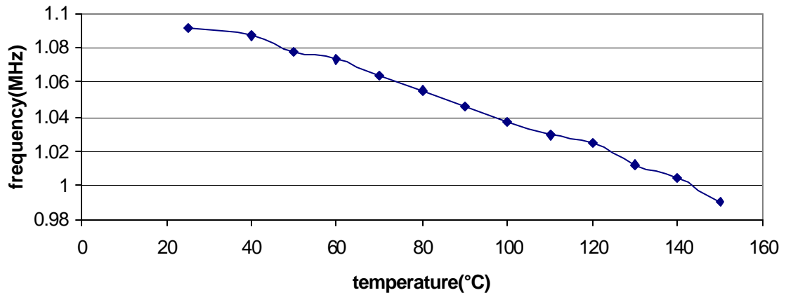
Fig.4 Frequency vs temperature
