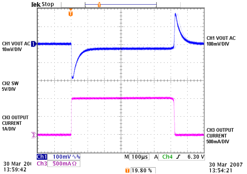
Fig.7 1A transient response
