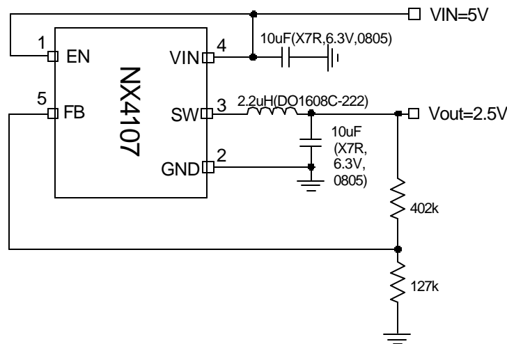
Figure1 - Typical application of NX4107CZ1TR
