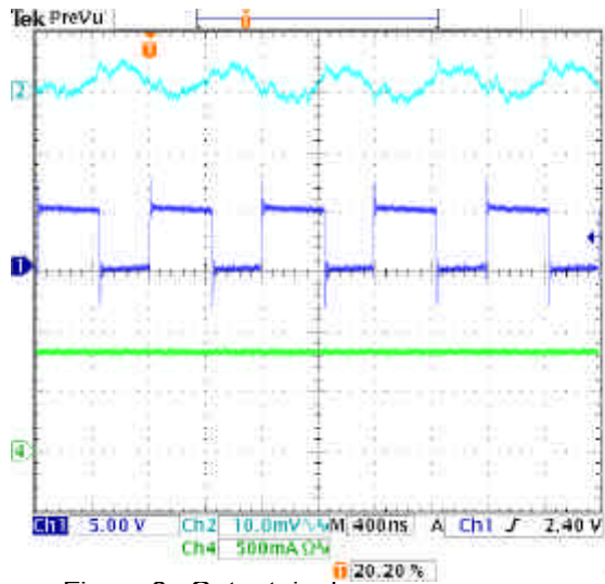
Figure 6 - Output ripple
