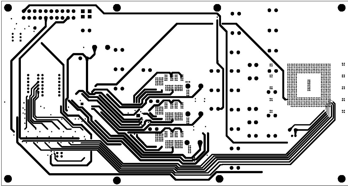
L3 POWER PLANE
