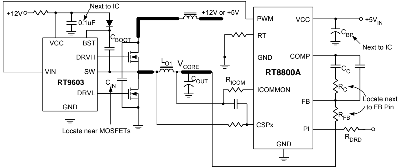
Figure 19. Layout Consideration
