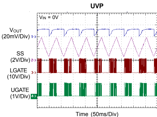
Figure 12. UVP (Always Hiccup Mode)
