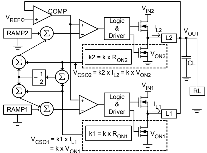
Figure 5. Current Balance
