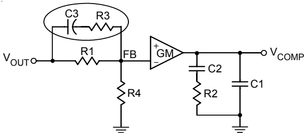
Figure 9. Additional Network of Type 3 Compensation (Add between V_{OUT} and FB)
