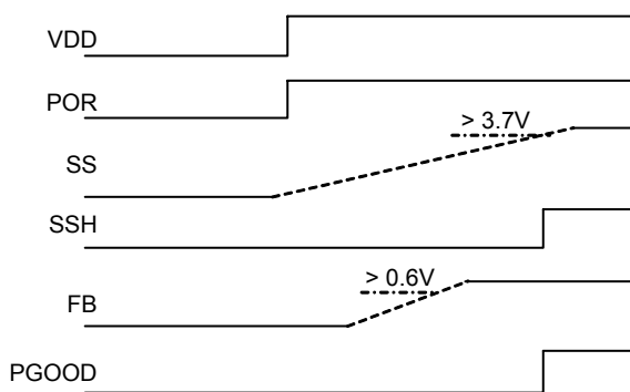
Figure 1. Power Sequence
