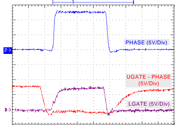
Time (100ns/Div) V_{CC} = 8V , 20MHz bandwidth limited
