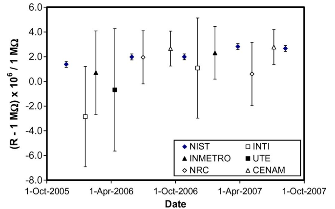
Fig. 4. Reported resistance and expanded uncertainty ( k = 2 ) for a 1 \text{ M}\Omega standard resistor. Each data point represents the mean of several weeks of measurements by the pilot or a participant laboratory. Similar data were observed for the other 1 \text{ M}\Omega resistor.
