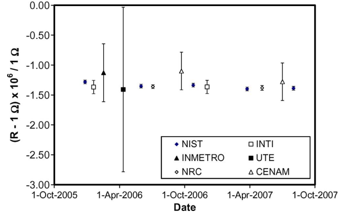
Fig. 3. Reported resistance and expanded uncertainty ( k = 2 ) for a 1 \Omega standard resistor. Each data point represents the mean of several weeks of measurements by the pilot or a participant laboratory. Similar data were observed for the other 1 \Omega resistor.
