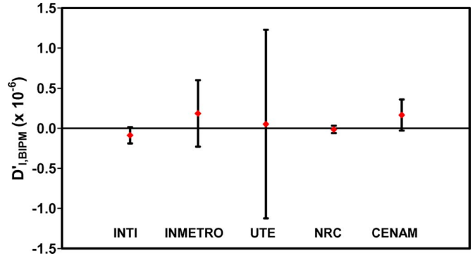
Fig. 9. Graph of equivalence at 1 \Omega that links the regional comparison SIM.EM-K1 to the bilateral comparison BIPM.EM-K13a. The NIST is the linking laboratory. The graph shows the differences from the BIPM.EM-K13a bilateral CRV. The error bars denote the expanded uncertainty ( k = 2 ) for each measurement laboratory with respect to the bilateral CRV.
